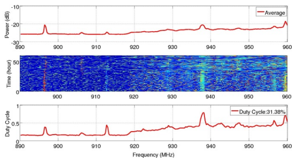
Fig. 9: Duty cycle and spectrogram of GSM 900 band
