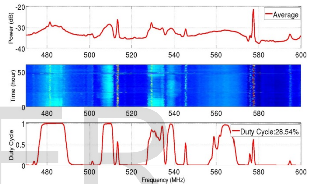
Fig. 6: Duty cycle and spectrogram of TV band 470 to 600 MHz
